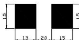
● Recommended Soldering Pattern
