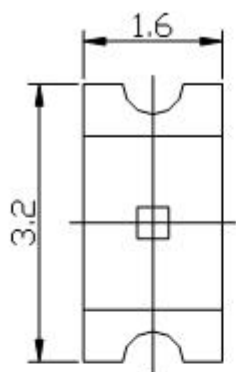
Package Outline Dimensions:
